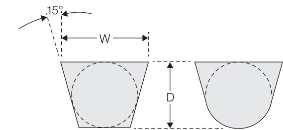
Figure 15: Trapezoidal runner profiles
