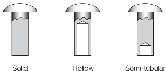
Figure 33: Example rivets
